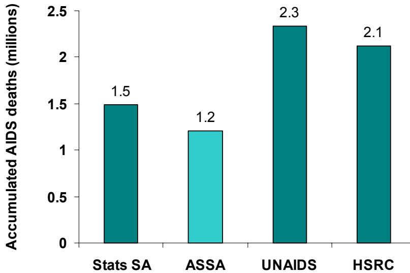
Figure 8. Accumulated number of AIDS deaths to middle 2004
